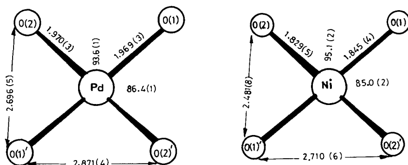
FIGURE 2 Coordination polyhedron around the metal atom.
