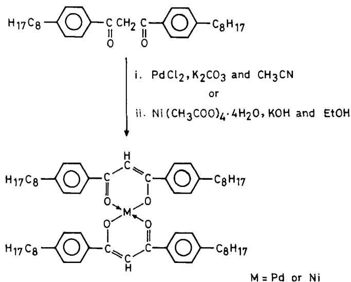
FIGURE 1 Synthetic route.
